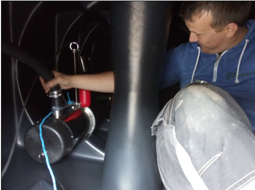
Securing the Hose to the Hosetail inside the Tank prior to final placement of the SteelPump at the base of the Tank (note float switch is now Mac3 Key – Blue and Yellow)
