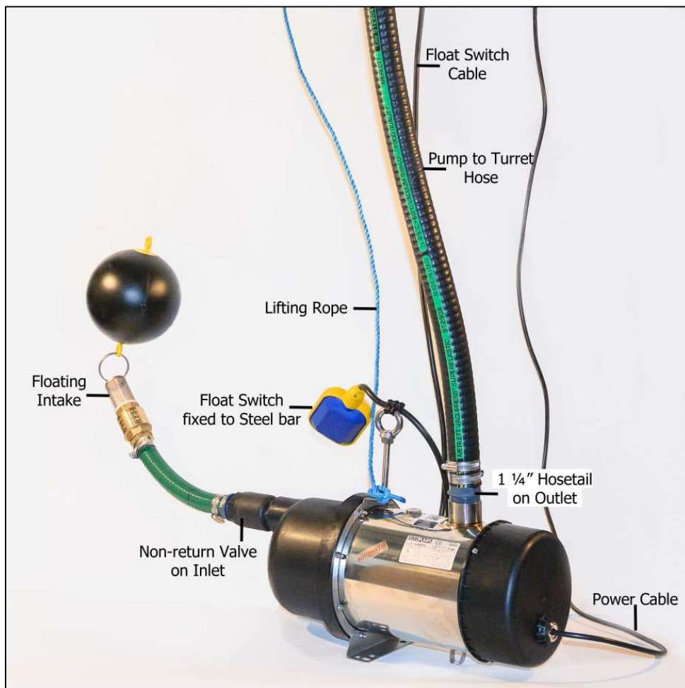
SteelPump assembly prior to placing inside the Tank
